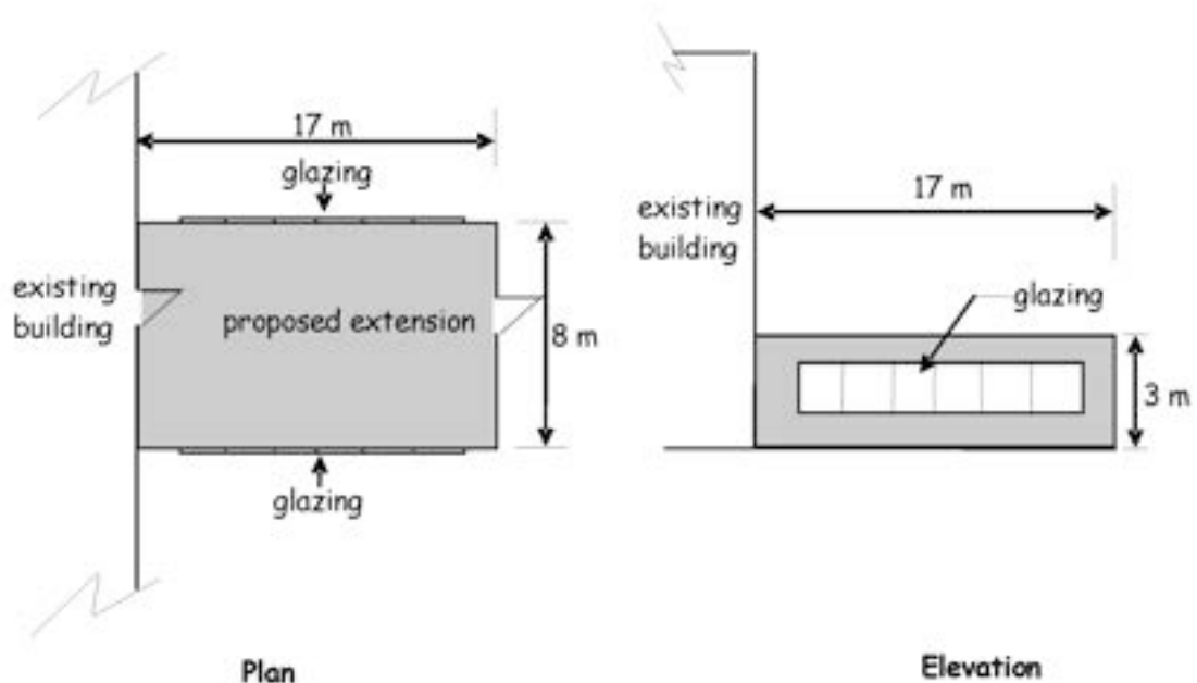
Figure 6.1 Extension example
