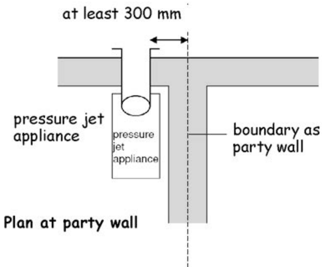
Figure 3.54 Separation between a boundary and terminal at right angles
