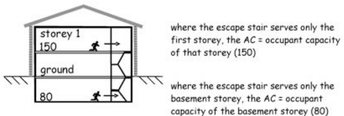
Figure 2.12 One storey example
