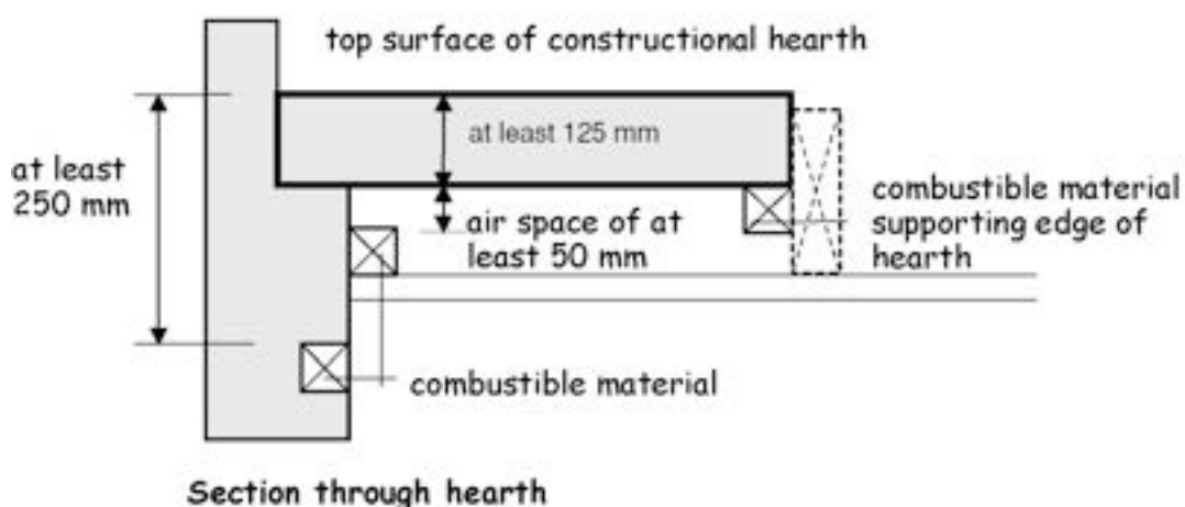
Figure 3.47 Section through hearth
