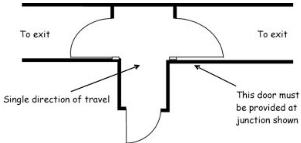
Figure 2.10 Corridor division
