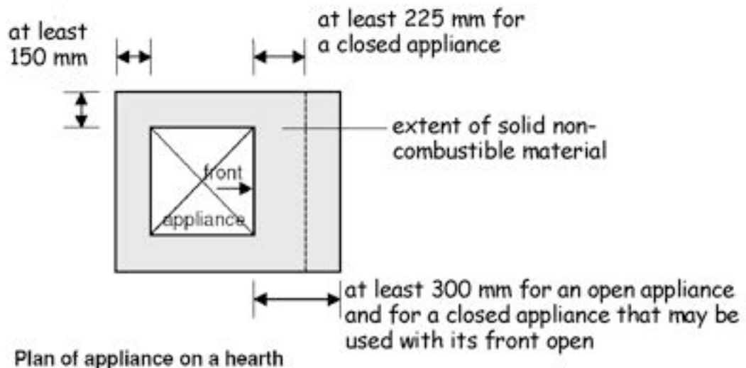
Figure 3.41 Appliance location
