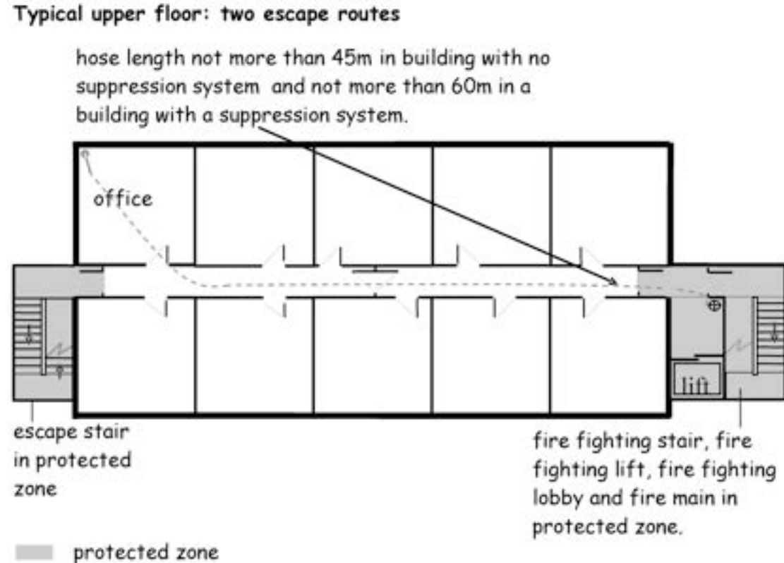
Figure 2.21 Two Escape Routes
