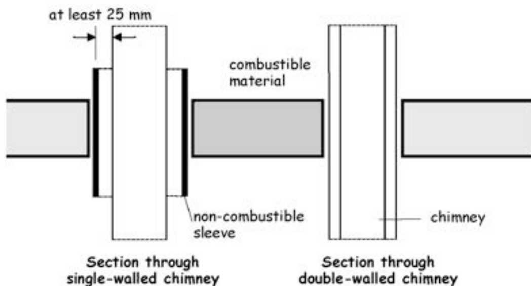
Figure 3.37 Section through single-walled chimney (vertical)
