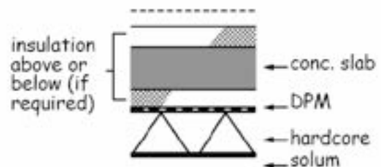
Figure 3.2 Ground supported concrete floors 2
