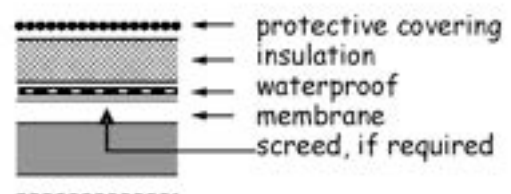
Figure 3.20 Roof constructions - Type B
